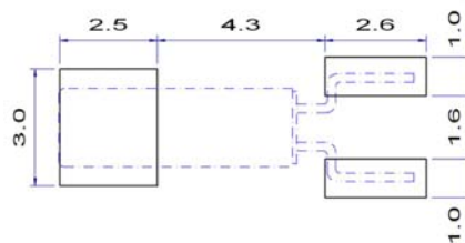
Example for soldering pattern
