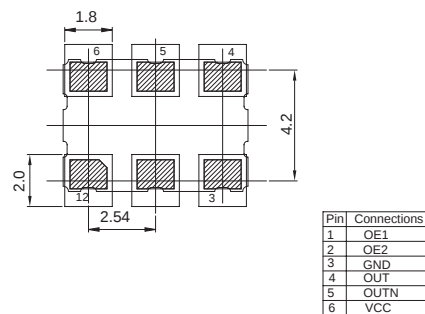
Recommended Land Pattern (mm) <Top View>
