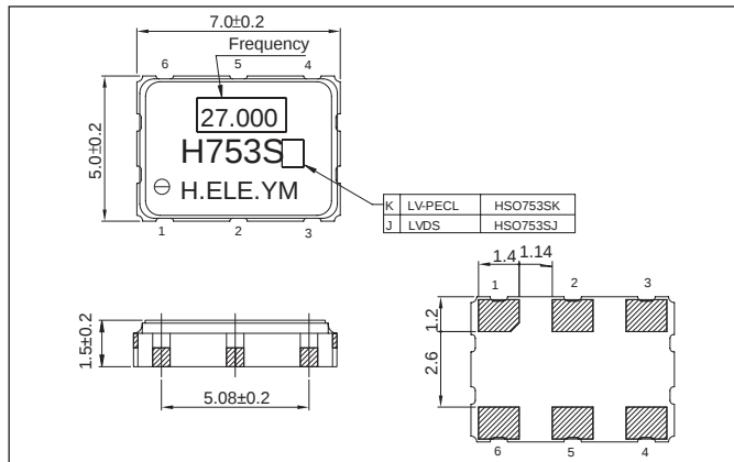
Recommended Land Pattern (mm) <Top View>
